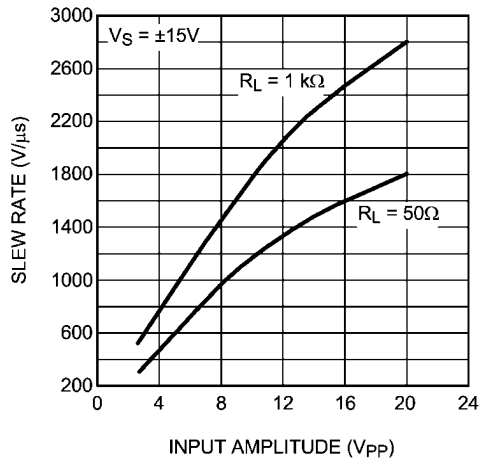
Slew Rate
