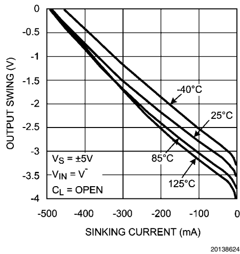
Negative Output Swing vs. Sinking Current
