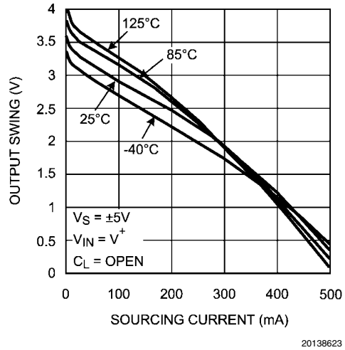
Positive Output Swing vs. Sourcing Current
