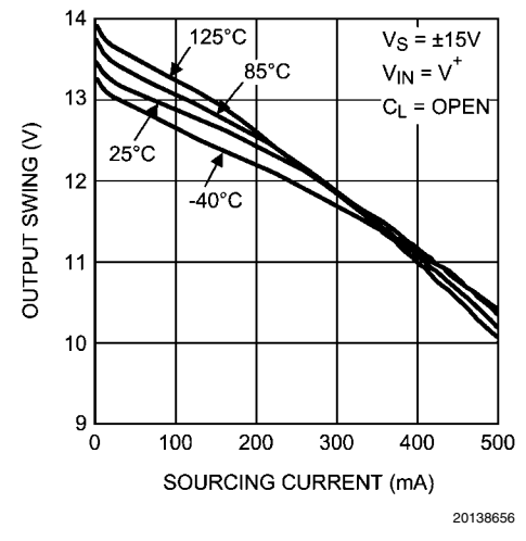
Positive Output Swing vs. Sourcing Current
